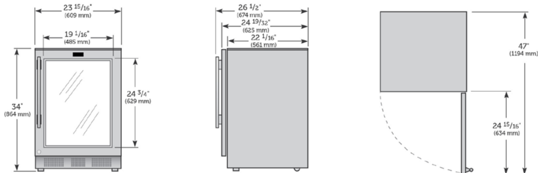
Height Dimensions +/- 1/2"
